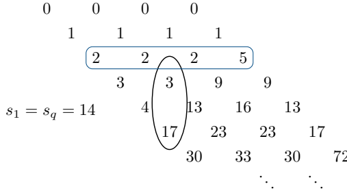
FIGURE 5. The 4-periodic infinite frieze associated to the quiddity sequence q = (2, 2, 2, 5) , with growth coefficient s_1 = 14 .
