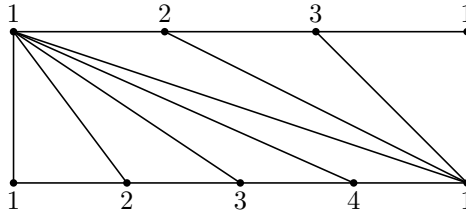
FIGURE 6. The triangulation giving rise to the frieze in Figure 5.
