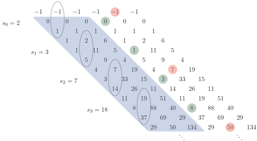
FIGURE 2. Growth coefficients (and the associated recursions) in the lattice of a periodic infinite frieze.
