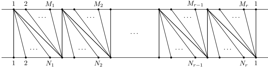
FIGURE 4. The fundamental domain of a bridging triangulation of A_{n,m} .
