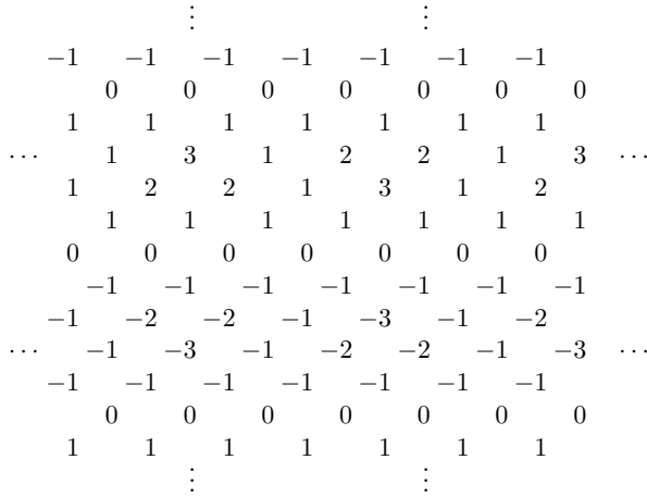
FIGURE 1. A lattice of a finite frieze.
