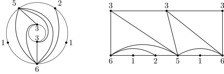
FIGURE 3. A triangulation of A_{5,2} providing outer quiddity sequence q = (6, 1, 2, 5, 1) and inner quiddity sequence \bar{q} = (3, 3) .
