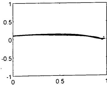
Figure 2: Solid line precise solution
