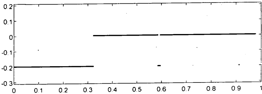
Figure 1: Piecewise constant optimal control
