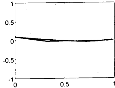
Figure 3: Solid line precise solution
