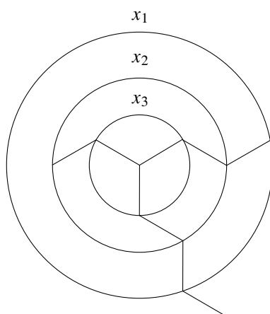
Figure 3 An example for Hurwitz's characterization.
