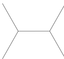
Figure 5 The two categories of isomers having exactly four primary carbons.
