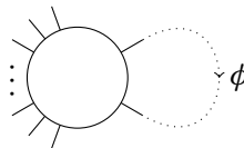
Figure 9. A self-gluing of X_{1,s}
