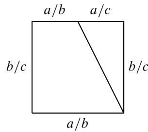
Figure 14. The parameter space, a punctured torus
