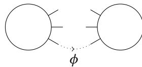
Figure 8. Gluing two copies of X_{1,3}
