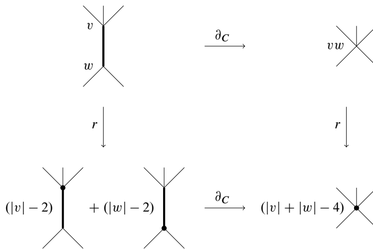
Figure 4. Diagram commutes because |vw| = |v| + |w| - 2
