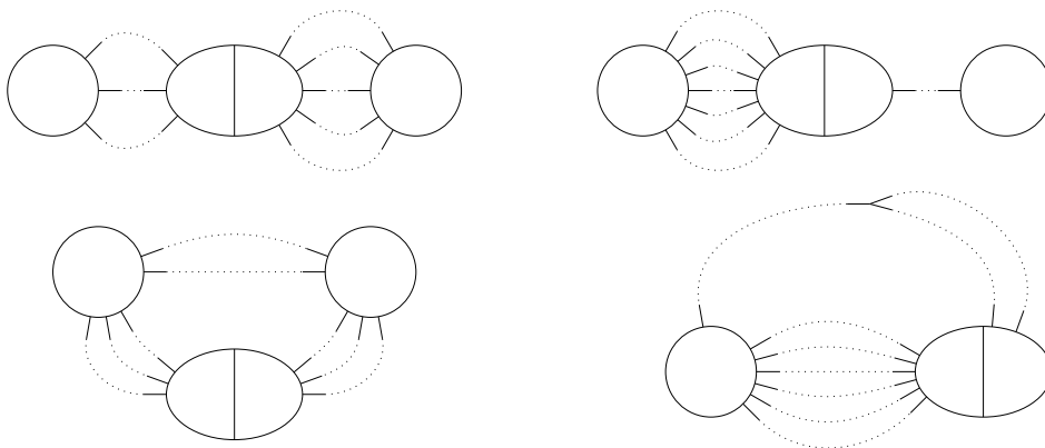
Figure 12. Candidates for a nontrivial class in H_{15}(\text{Out}(F_{10}))
