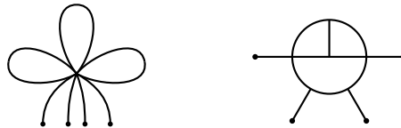
Figure 3. Two possibilities for X_{3,4}
