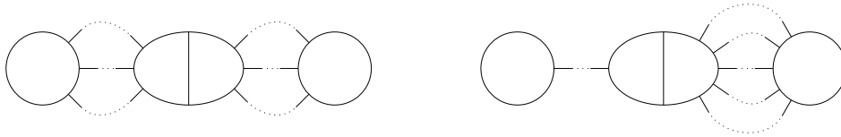
Figure 11. Candidates for a nontrivial class in H_{11}(\text{Out}(F_8))
