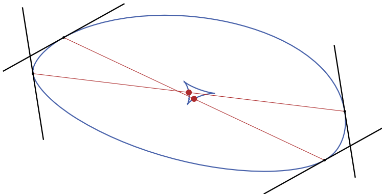
Figure 3. Midpoints of diameters trace out the centrix.
