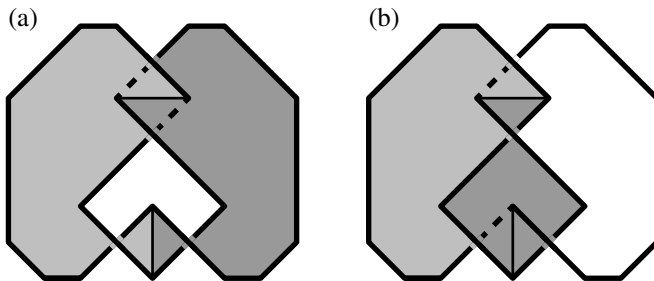
Figure 4. The figure-8 knot complement equipped with (a) a full internal hyperbolic Mom-2 structure, and (b) a non-full internal Mom-2 structure with a non-hyperbolic underlying submanifold M .
