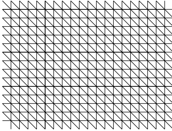
Figure 0. Hexagonal 3-web
