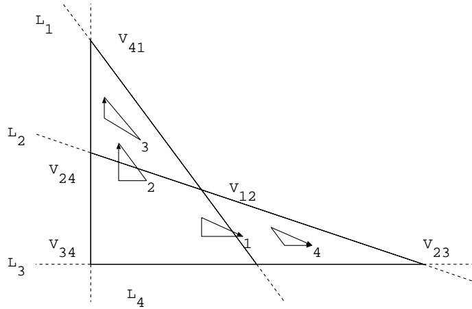
Figure 3. Schläfli configuration
