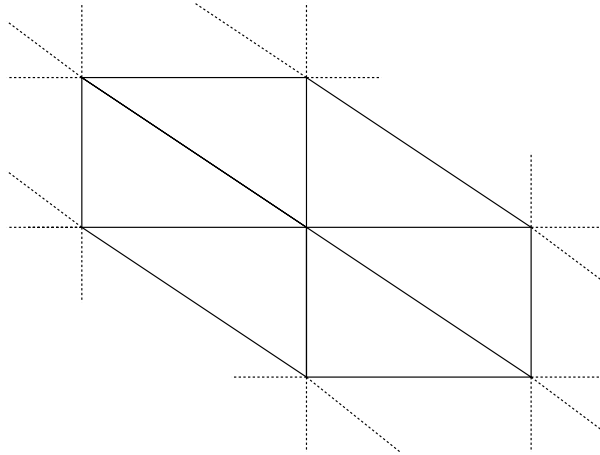
Figure 5. Closed hexagon
