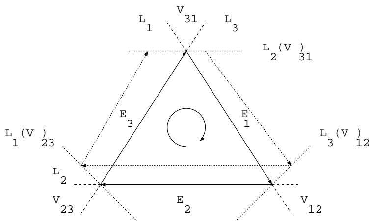
Figure 7. Fake billiard T_{\partial\Delta}^1
