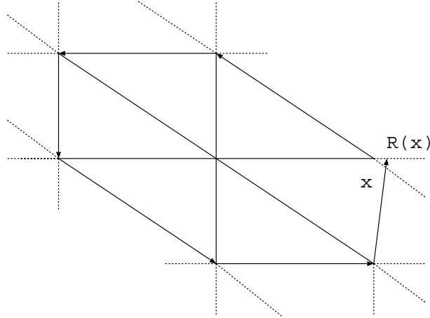
Figure 6. Non-closed hexagon
