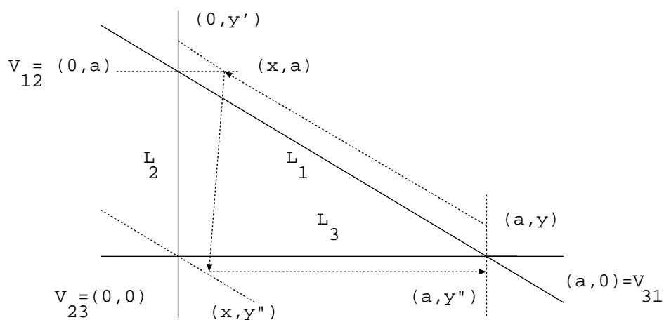
Figure 8. Fake billiard T_{\partial\Delta}^1 along another triangle
