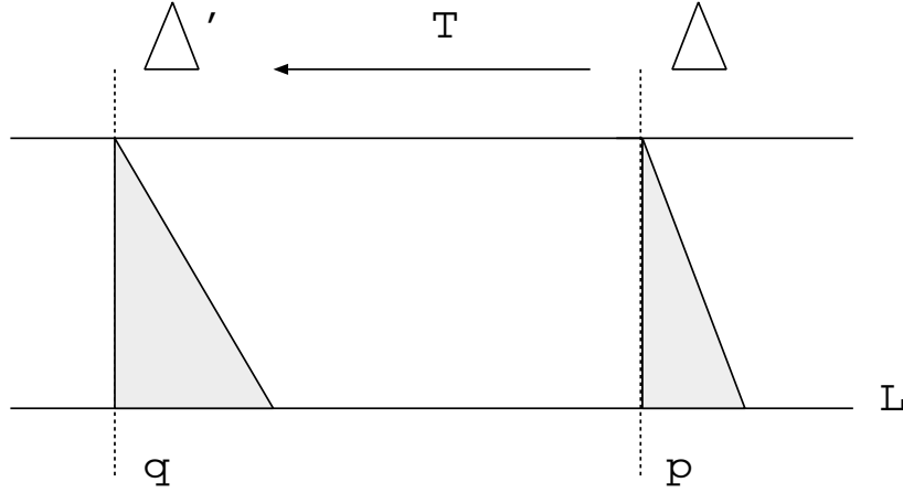
Figure 4. Transverse dynamics and Bott connection
